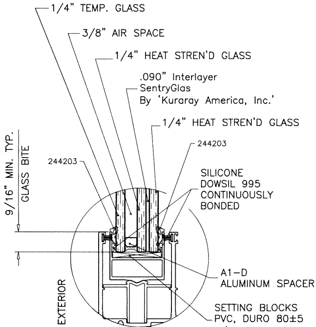
GLASS TYPE 'Bi'
