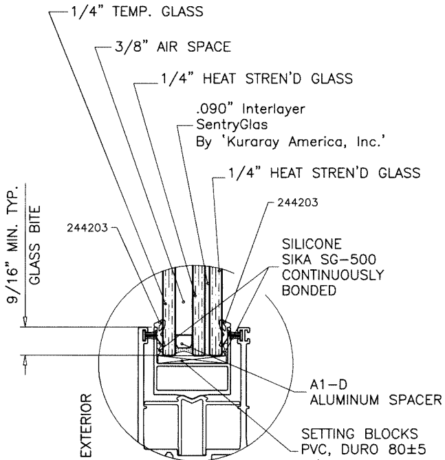
GLASS TYPE 'Ci'
